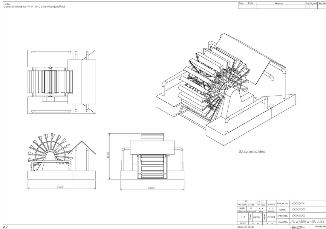
Rajah 4: Rajah Ringkas Sistem 'Micro Hydro Water Wheel'
