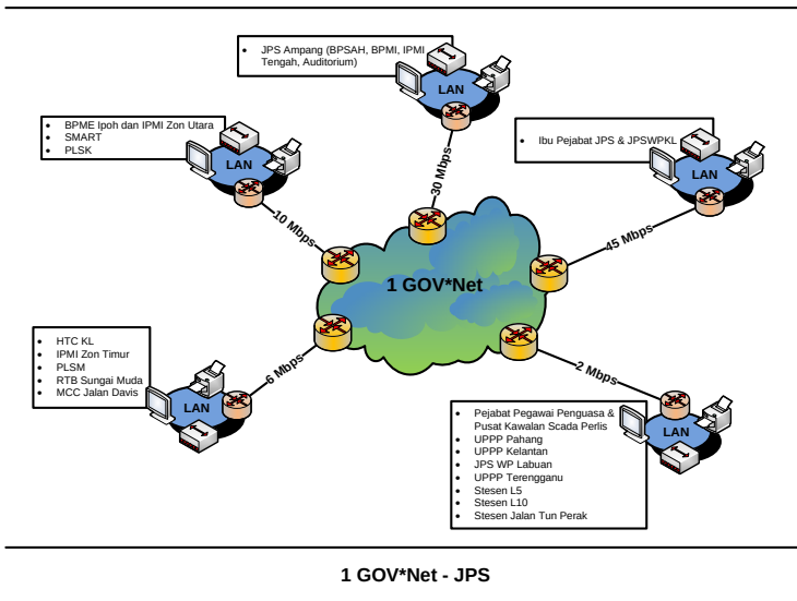
Gambarajah 17.1: Rangkaian JPS*Net
